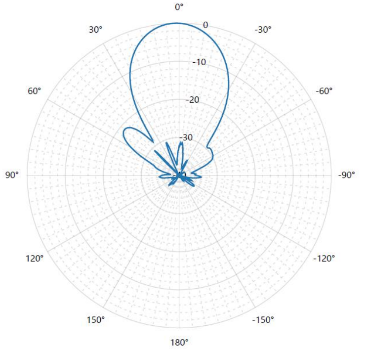
50 kHz 28° @ -3db
