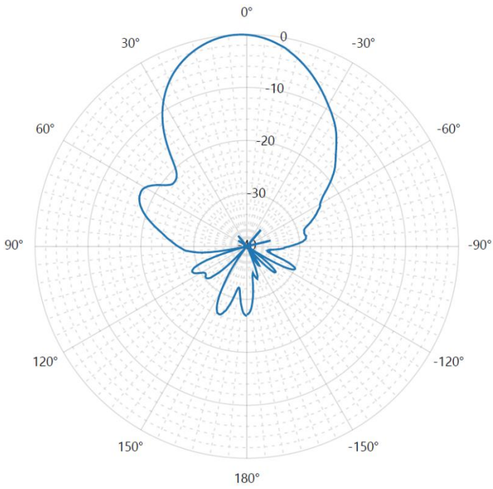
40 kHz 33° @ -3db
